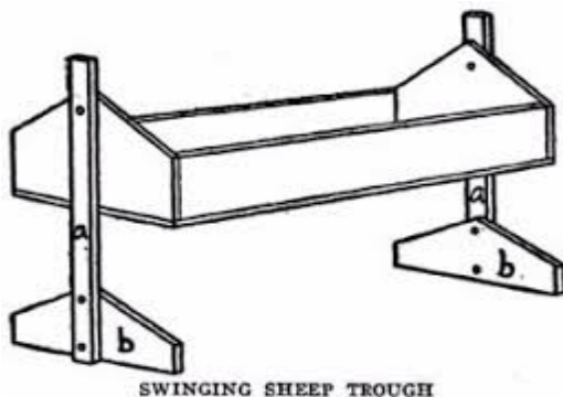
A structure of a feeding trough
